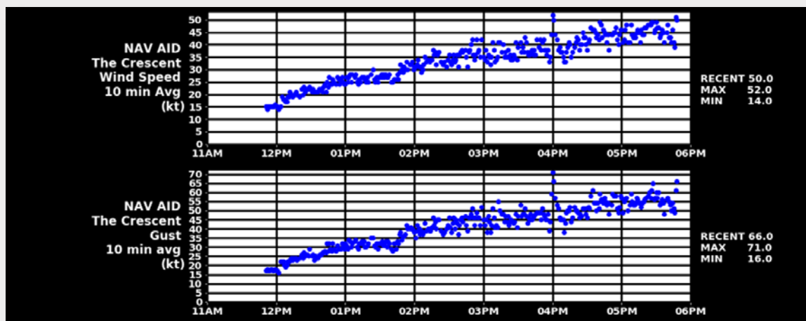
Developing gale near Bermuda, 28 January 2021 – Top left: model representation of wind speeds (shaded – red displays gale-force winds) at 2:00 PM (local time) on 28 Jan 2021 and sea level pressure (solid lines); red dot is the location of Bermuda. Top right: Satellite image for same time, with Bermuda highlighted. Bottom panels: Graph of sustained wind speeds and gusts measured at the Crescent navigation aid north of Bermuda on 28 January 2021 11:00AM to 6:00 PM (local time). Sustained winds reached gale force at approximately 2:00PM.
