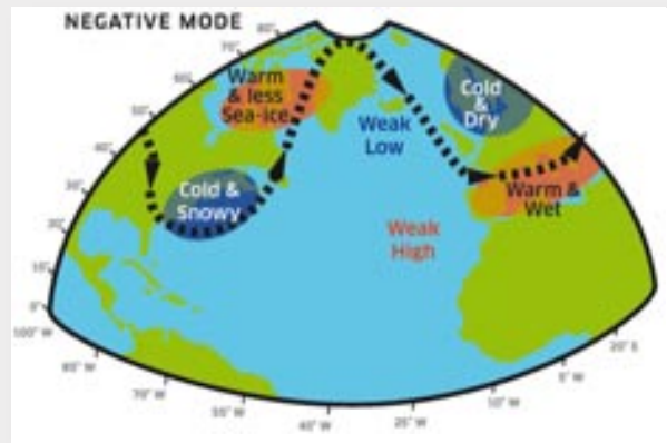
Figure 4: Number of rain days in Bermuda during winter (December through March), and the NAO Index for the same period, during the years 1949 to 2011 (top) - data from BWS, adapted from Peñate De La Rosa (2015). b) Schematic diagram of the positive (left) and negative (right) phases of the North Atlantic Oscillation (NAO), and their associated weather patterns (bottom). From Hughes et al. (2018)
