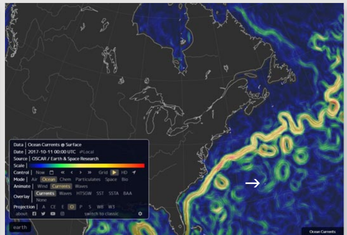
Left - Sea surface height anomaly map for 10 October 2017; Middle - Model ocean Currents with sea surface temperature anomaly for 11 October 2017; Right - Model surface current speed for 11 October 2017. White arrows indicate location of Bermuda. Source: US Navy, earth.nullschool.net
