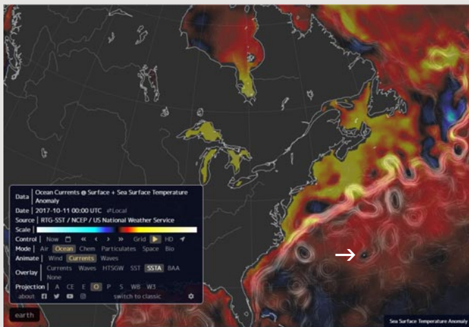
Left - Sea surface height anomaly map for 10 October 2017; Middle - Model ocean Currents with sea surface temperature anomaly for 11 October 2017; Right - Model surface current speed for 11 October 2017. White arrows indicate location of Bermuda. Source: US Navy, earth.nullschool.net
