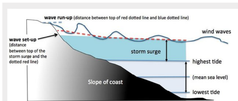
Schematic of different elements of storm tide. Source: Australian Government National Climate Change Adaptation Research Facility.
