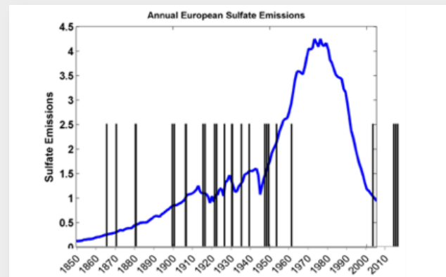
The blue graph indicates European sulphate aerosol (pollution) emissions in 1000s of metric tonnes (Smith et al., 2011), overlaid upon instances of major hurricanes within 200 km of Bermuda, through the historical record (NOAA).
