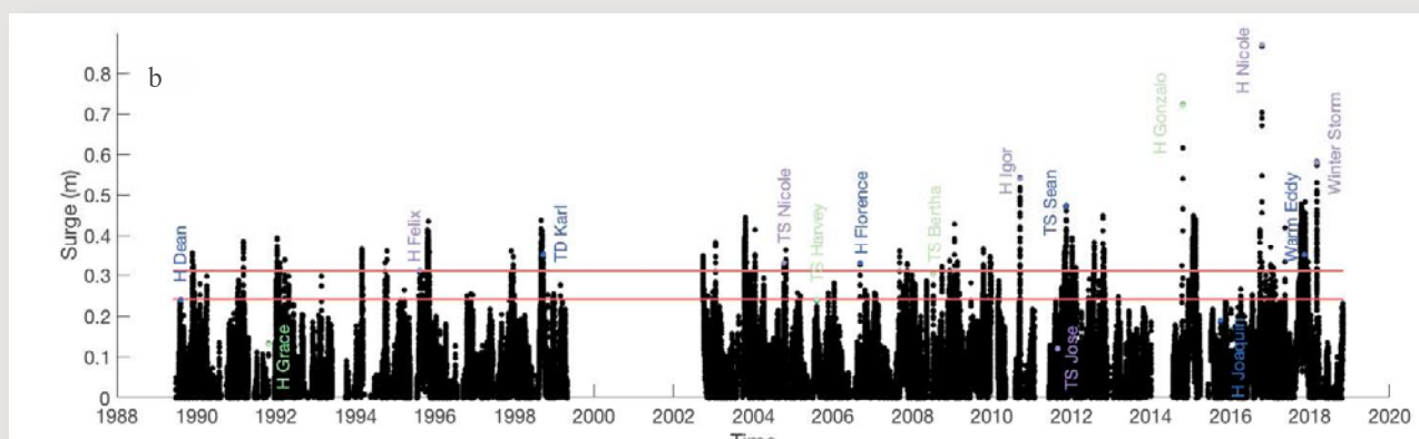
Figure 4 Time series of positive surge from the St. George's, Bermuda tide gauge, from June 1989 until October 2018. 14 selected TS and H events and two non-hurricane events (i.e., winter storm and a warm eddy) are incorporated within the time-series.
