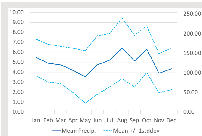
Figure 1. Average (1981-2020) Bermuda’s monthly precipitation (solid blue line), +/- standard deviation of the monthly mean (dashed light blue line). Measurements are displayed in inches (left axis) and mm (right axis). Data from www.weather.bm/climate.asp - all measurements taken at LF Wade International Airport by BWS.
