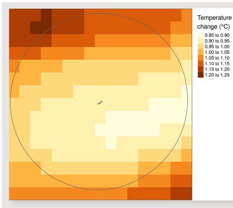
Map of temperature change 2025 - 2095. This is the mean of the annual epipelagic temperature data for 2091-2100 minus the mean of the annual data for 2021 - 2030 (see following figure for those individual maps). Circle shows the boundary of Bermuda's Exclusive Economic Zone, and the land mass is shown in black in the middle. Graphic courtesy of Jason Flower, UCSB, 2022, using data from Brito-Morales et al. (2022)
