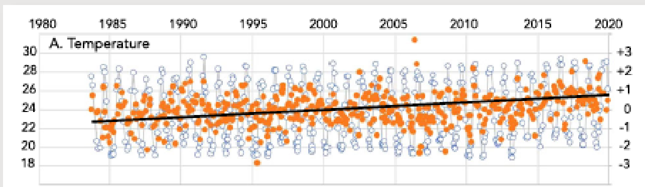
Observed ocean surface temperature and anomalies (°C) (left vertical axis; open blue symbols); anomalies and linear regression of anomalies (right vertical axis; orange symbols). Figure from (Bates & Johnson, 2020), their Fig.1 a, reproduced under Creative Commons Attribution 4.0 International License.
