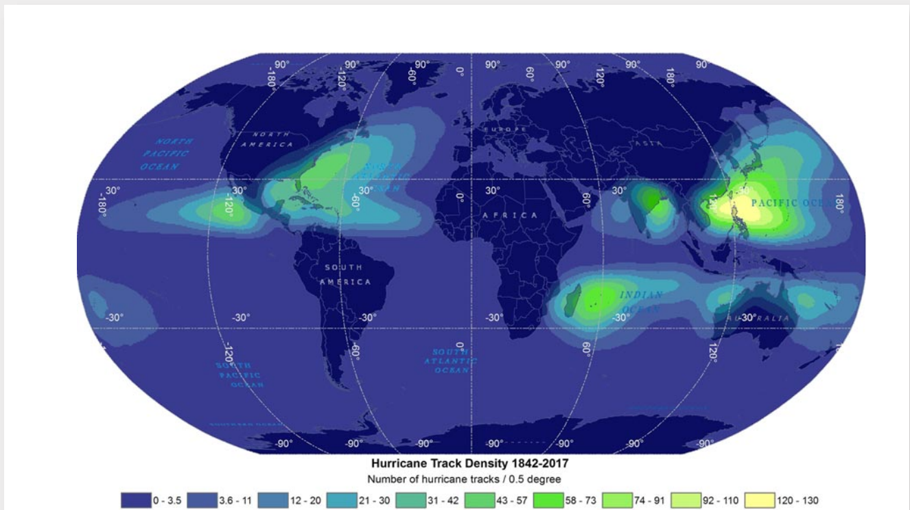
Locations of tropical cyclone tracks from 1842 to 2017. Data Source: NOAA International Best Track Archive for Climate Stewardship (IBTrACS)
