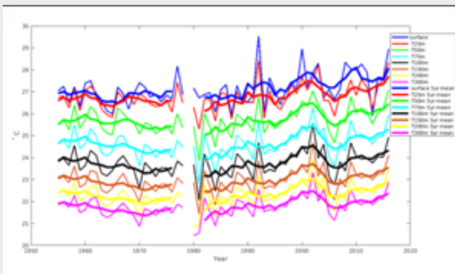
Average August, September and October upper ocean temperatures averaged down to different depths (32°N, 64°W). Note the warming trend through the decades (Hallam et al., 2021).
