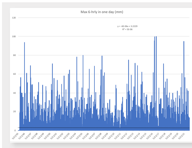
Figure 5. Maximum six-hourly rainfall accumulations (top) measured by BWS, June 1995-March 2022, and rolling 365-day standard deviation of the maximum six-hourly accumulations (bottom).
