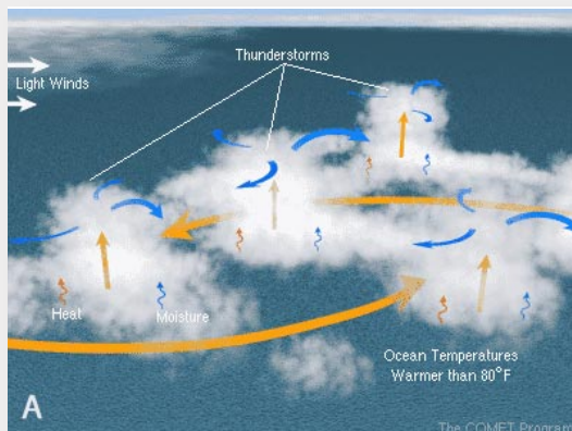
Schematic depiction of A) Precursor conditions leading to B) development of a hurricane (cross-section). Image Source: University Corporation for Atmospheric Research (UCAR) - COMET Program, courtesy of NASA
