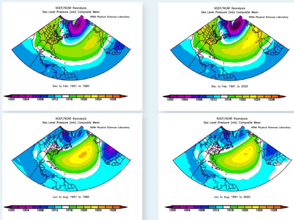
North Atlantic mean sea level pressure for (Top panels) winter months (December-February) and (Bottom panels) summer months (June-August) compared between (left panels) the averages for all the years 1951-1980 and (Right panels) the averages for the period 1991-2020 (data: NCEP/NCAR Reanalysis (Kalnay et al., 1996)).
