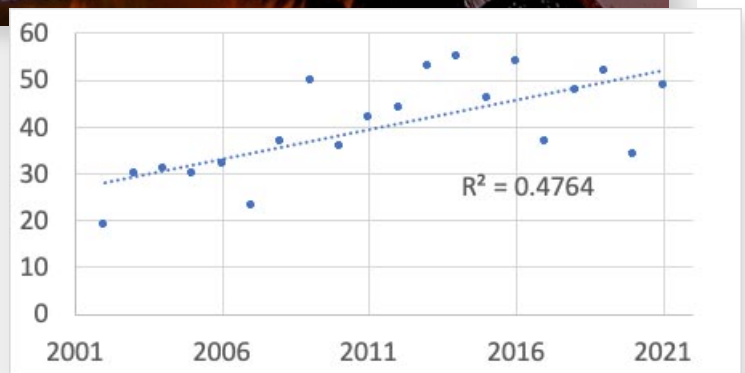
Number of days per year on which thunder was reported at LF Wade International Airport 2002-2021. Source: BWS.
