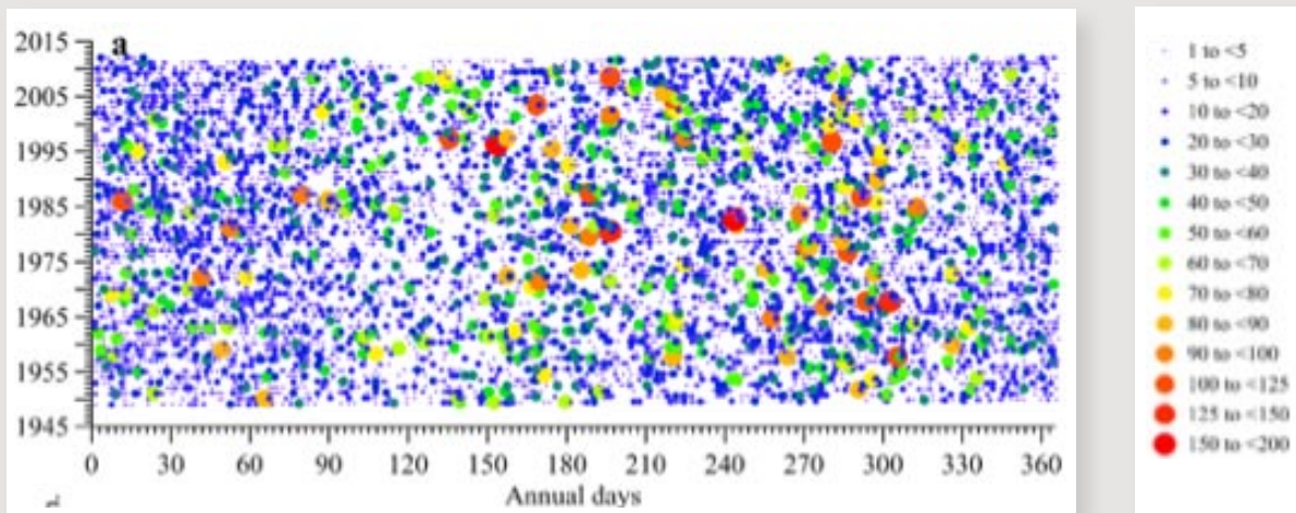
Figure 2. Annual and interannual variability of rainfall in Bermuda. Daily occurrence of rainfall on a day in a given year; intensity is given by colour and circle size, in mm/day. Daily data from BWS, for 1949 to 2011.
