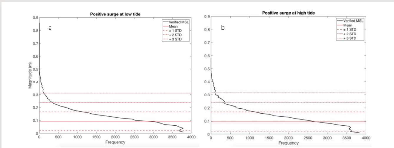
Figure 3. Frequency of positive surge levels with statistical analysis (mean, one, two, and three \sigma ) at (a) low tide and (b) high tide.
