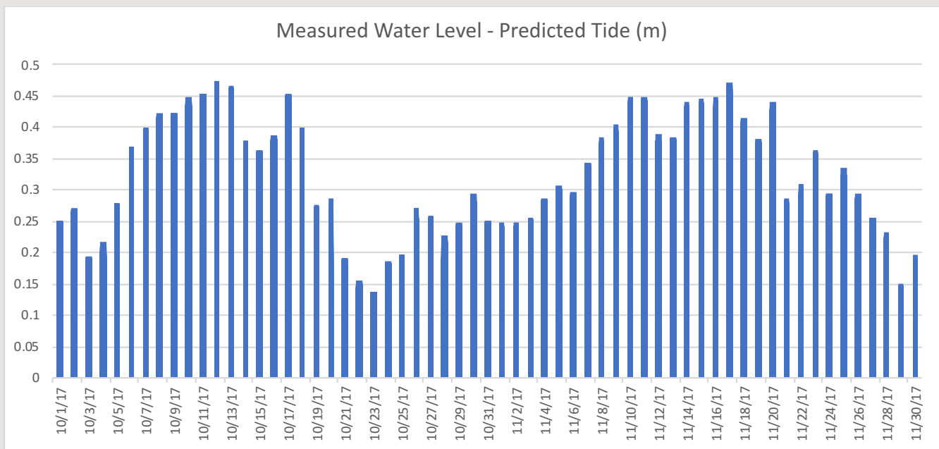
Water level departures above the normal (predicted) tide levels for October through November 2017 at the NOAA Tide Gauge on the north side of St. George's
