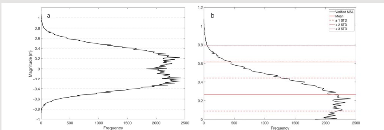
Figure 2. (a) Frequency of all verified water levels and (b) frequency of positive verified water levels with statistical analysis (mean, plus one, two, and three standard deviations [STD]).
