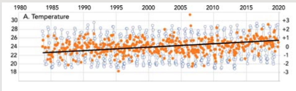
Observed data (left vertical axis; open blue symbols) and anomalies (right vertical axis; orange symbols) are shown. Regression lines are from anomaly data plotted in the right vertical axis. a Surface temperature and anomalies ( ^{\circ}\text{C} ).
