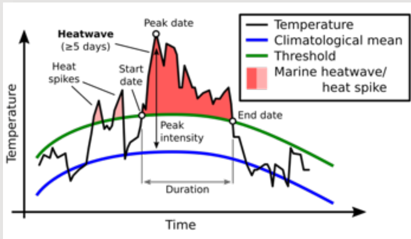
Figure 1. a) A marine heatwave is defined as when seawater temperatures exceed a seasonally-varying threshold (usually the 90th percentile) for at least five consecutive days. Successive heatwaves with gaps of two days or less are considered part of the same event. Source: www.marineheatwaves.org/all-about-mhws.html .
