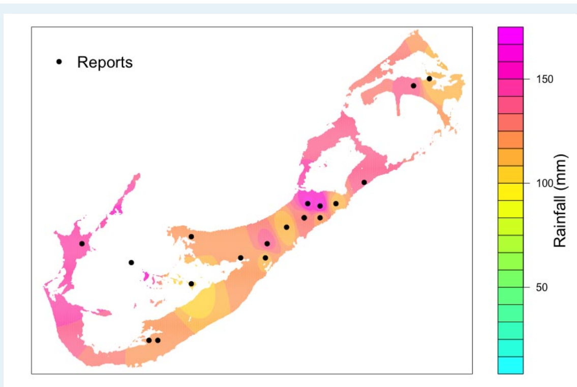
Rainfall accumulations over 24 hours from different private and public sites around the island – adapted from Johnston et al. (2018). Note the high variability of rainfall amounts in different parishes.
