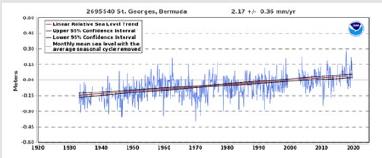
Figure 1. Annual MSL trend (1932-2019) based on NOAA's tide gauge at St. George's https://tidesandcurrents.noaa.gov/sltrends/sltrends_station.shtml?id=2695540 - this is referenced to a 1983-2001 Mean Sea Level datum. Middle panel: Annual MSL trend (1932-2019) and future projections of sea level rise for Bermuda (Kopp et al. 2014a) for Representative Concentration Pathway (RCP) 2.6, 4.5, and 8.5. (a) Dashed: low-sensitivity; solid: mid-sensitivity; dotted: high-sensitivity sea level projections; (b) RCP 2.6 at low-sensitivity, RCP 4.5 at mid-sensitivity, and RCP 8.5 at high-sensitivity; (c) Coastal Risk Screening Tool - Land projected to be below annual flood level in 2050 - https://coastal.climatecentral.org/ - accessed 31 March 2022.
