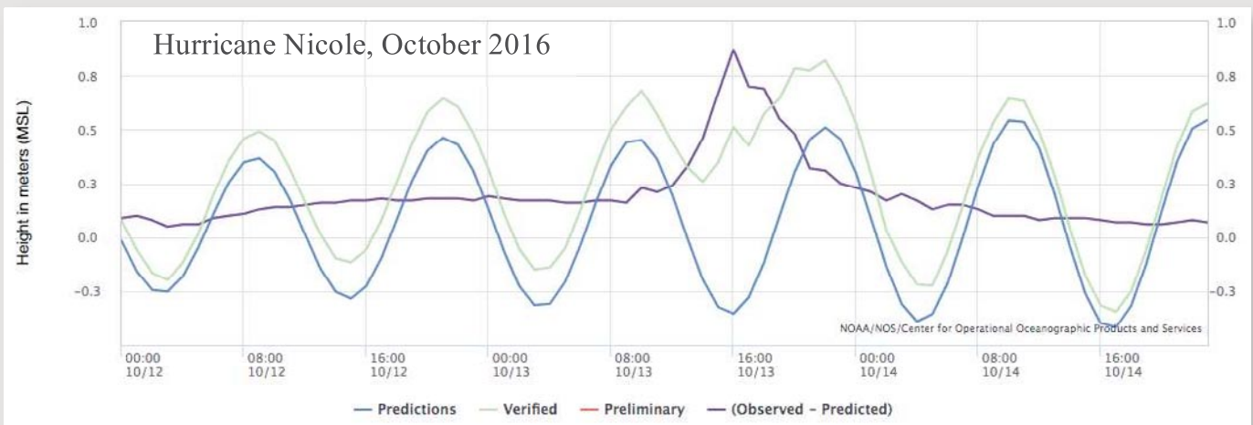
Figure 5. Example of tide gauge data from 12 to 14 October 2016 to show the water levels in Bermuda when Hurricane Nicole occurred.
