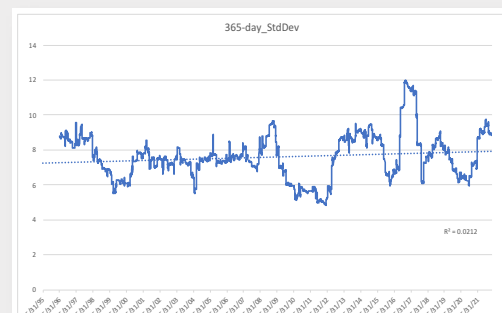
Figure 5. Maximum six-hourly rainfall accumulations (top) measured by BWS, June 1995-March 2022, and rolling 365-day standard deviation of the maximum six-hourly accumulations (bottom).
