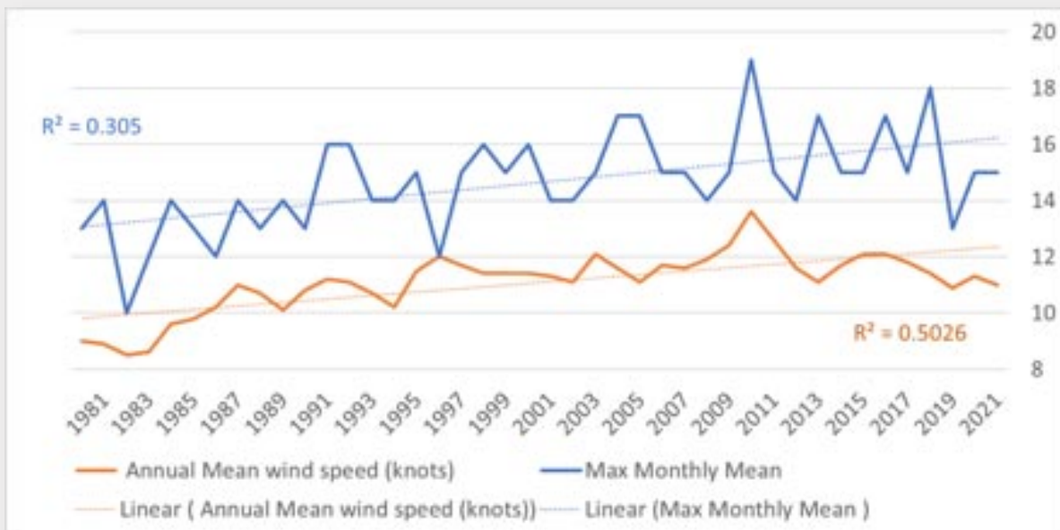
Average monthly wind speeds and maximum of monthly averages (both in knots), based on measurements at LF Wade International Airport 1980-2021. Data from Bermuda Weather Service, Bermuda Airport Authority. Linear trends and R2 values also shown.
