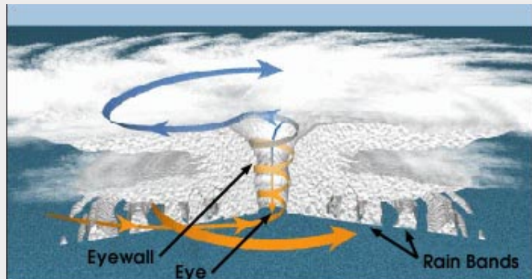
Schematic depiction of A) Precursor conditions leading to B) development of a hurricane (cross-section). Image Source: University Corporation for Atmospheric Research (UCAR) - COMET Program, courtesy of NASA
